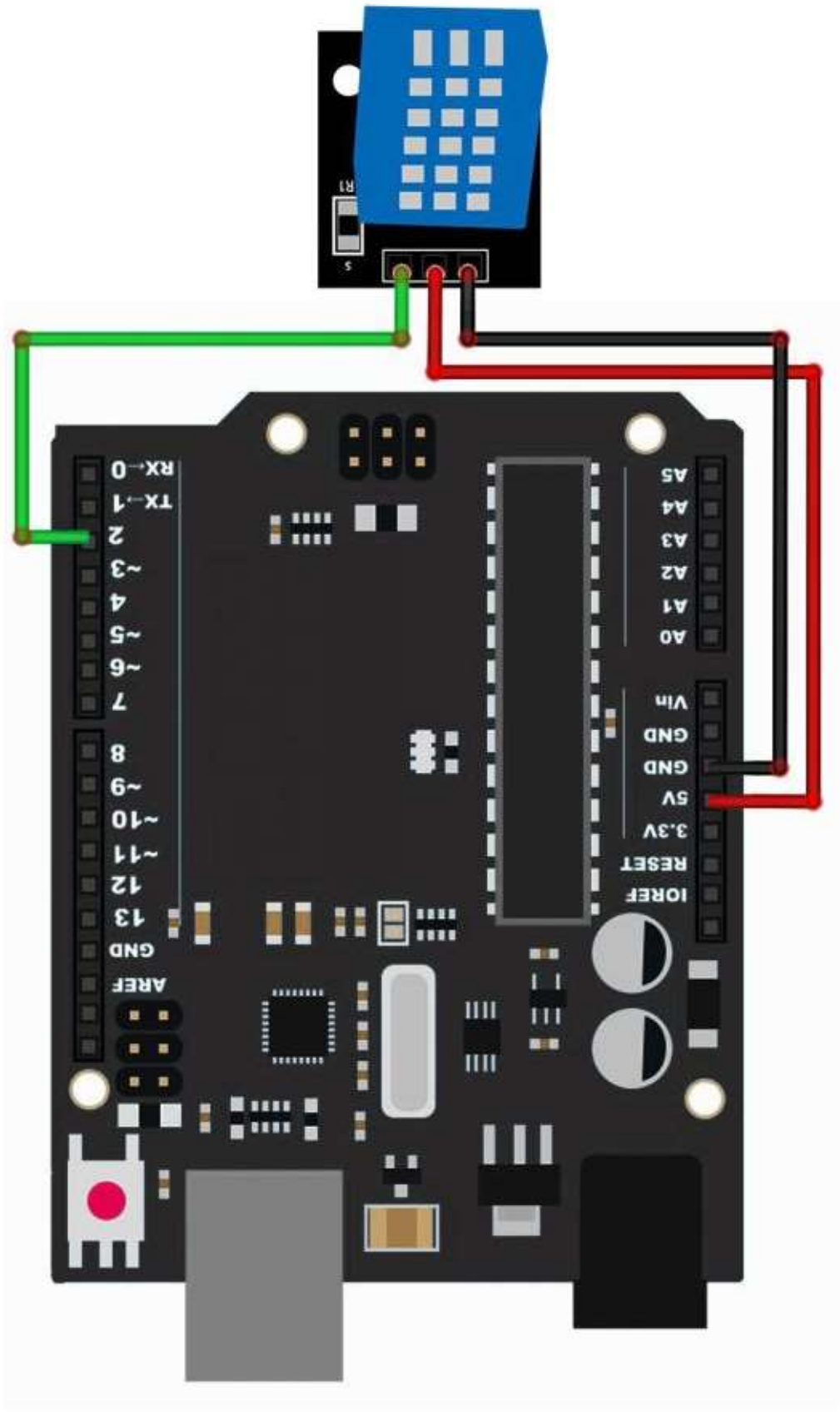
Wiring diagram
